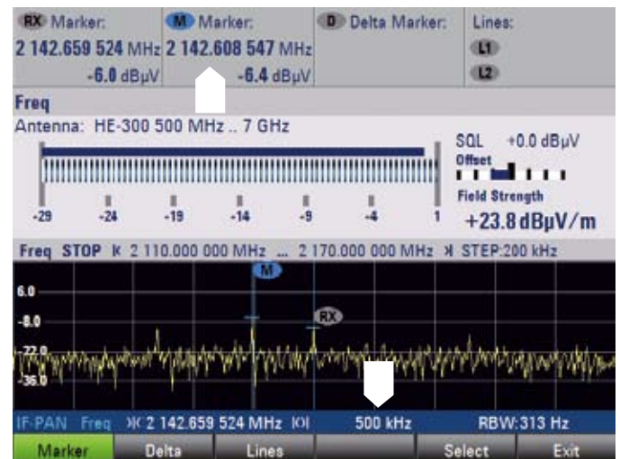
Marker menu selected: 2nd RFI signal IF realtime span of 500 kHz.
