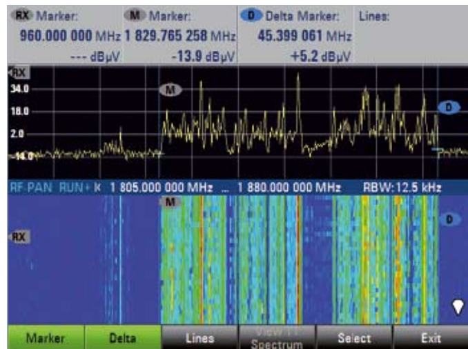
GSM1800 downlink band, markers active.
