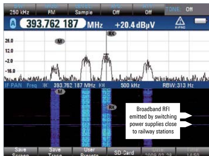
TETRA downlink band 4, four channels on air.
