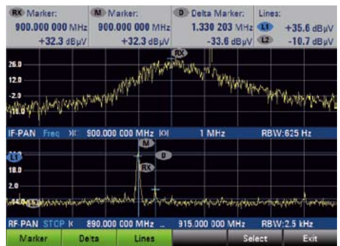
Interference from a broadband digital signal on the same GSM 900 MHz channel.
